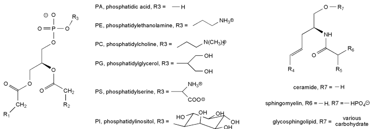
FIGURE 4. General structures of glycerophospholipids (left) and sphingolipids (right). For the glycerophospholipids, stereospecific sites on the glycerol backbone are numbered (“ sn ” numbering). R 1 and R 2 represent alkyl chains that may be saturated or unsaturated. Together with an attached —CH 2 CO— group, they constitute the “fatty acyl” chains at positions sn -1 and sn -2 of the glycerol backbone. The α methylene groups of these chains are depicted apart from the R groups because their hydrogen atoms participate in some of the decomposition reactions discussed in the text. The —CH 2 CO— group at sn -1 position is replaced with —O— in ether lipids, and with —CH=CH—O— in vinyl ether lipids or plasmalogens. The R 3 group defines the six major phospholipid headgroup classes. For sphingolipids, R 4 is usually —C 13 H 27 but may be —C 12 H 25 . The R 5 is an alkyl group ranging in length from 2 to 20 carbon atoms. R 6 may be —H or —OH.
