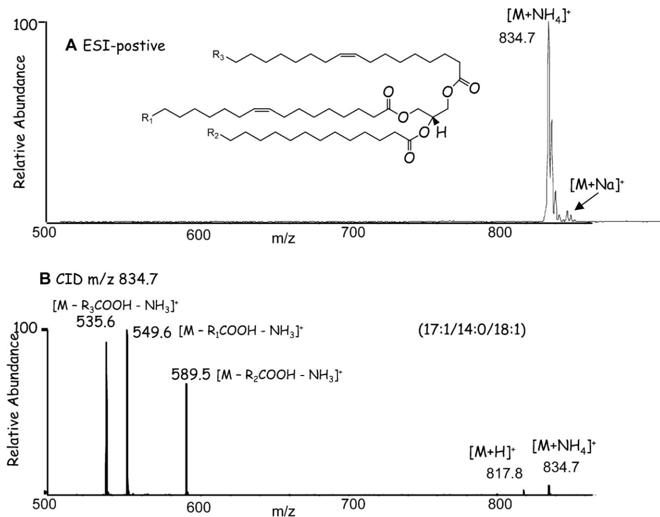
FIGURE 3. A: ESI in the positive ion mode of synthetic 17:1/14:0/18:1 triacylglycerol in the presence of electrospray buffer containing 5 mM ammonium acetate; (B) CID of [M + \text{NH}_4]^+ at m/z 834 resulting in indicated product ions corresponding to loss of each of the fatty acyl substituents as a free carboxylate anion.
