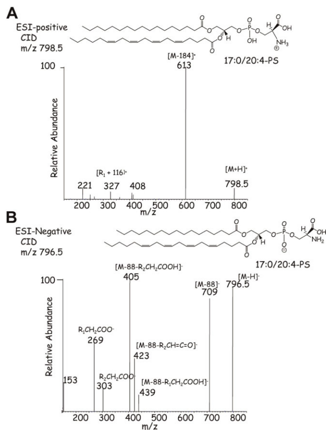
FIGURE 8. Positive and negative ion CID mass spectra from 1-heptadecanoyl-2-arachidonoyl-3-glycerophosphoserine (17:0/20:4-PS). Molecular ion species generated by ESI. A: Collisional activation of the [M + H]^+ ion at m/z 798.5; (B) Collisional activation of the [M - H]^- ion at m/z 796.5.
