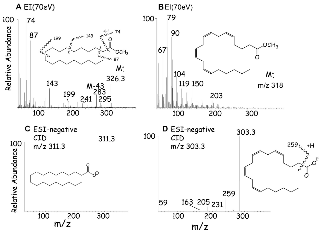
FIGURE 1. EI mass spectra of fatty acid methyl esters and collision-induced decomposition (CID) of carboxylate anions from free carboxylic acids. A: EI mass spectrum of methyl arachidate (70 eV); (B) EI mass spectrum of methyl arachidonate (70 eV); (C) CID mass spectrum of the carboxylate anion derived from arachidonic acid by ESI in the negative ion mode; (D) CID mass spectrum of the carboxylate anion derived from arachidonic acid by ESI in the negative ion mode. The CID mass spectra for this figure and subsequent figures were obtained using a tandem quadrupole (ABI 4000 Qtrap).
