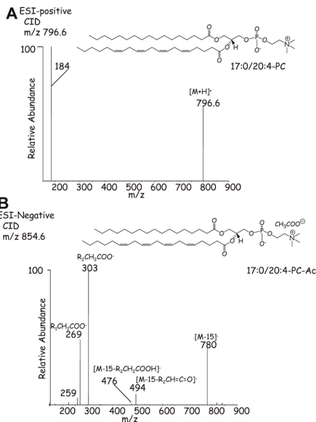
FIGURE 7. Positive and negative ion CID mass spectra from 1-heptadecanoyl-2-arachidonoyl-3-glycerophosphocholine (17:0/20:4-PC). Molecular ion species generated by ESI. A: Collisional activation of the [M+H]^+ ion at m/z 796.6; (B) collisional activation of the [M+acetate]^- ion at m/z 854.6.
