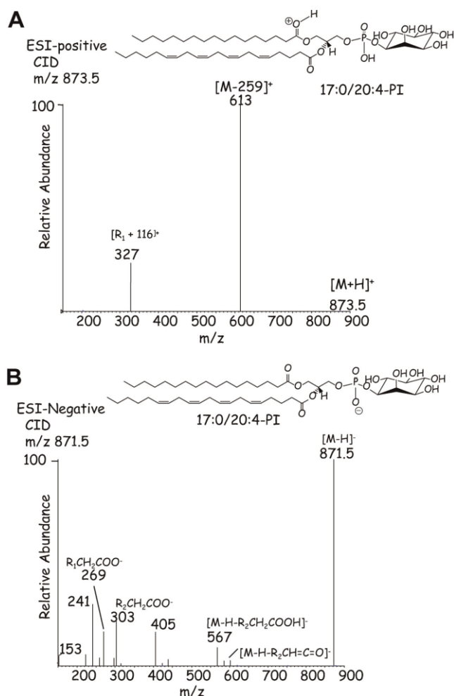
FIGURE 10. Positive and negative ion CID mass spectra from 1-heptadecanoyl-2-arachidonoyl-3-glycerophosphoinositol (17:0/20:4-PI). Molecular ion species generated by ESI. A: Collisional activation of the [M+H]^+ ion at m/z 873.5; (B) collisional activation of the [M-H]^- ion at m/z 871.5.
