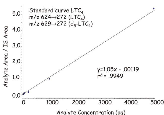
FIGURE 2. Quantitation by stable isotope dilution of lipids typically involves establishing a standard curve where a fixed amount of a deuterium-labeled internal standard (in this case d_5 -LTC 4 ) is added to increasing quantities of unlabeled LTC 4 . When the area for the MRM transition for LTC 4 ( m/z 624 \rightarrow 272) is divided by the area for the corresponding internal standard ( m/z 629 \rightarrow 272 for d_5 -LTC 4 ), a linear relationship is found with an excellent correlation coefficient.
