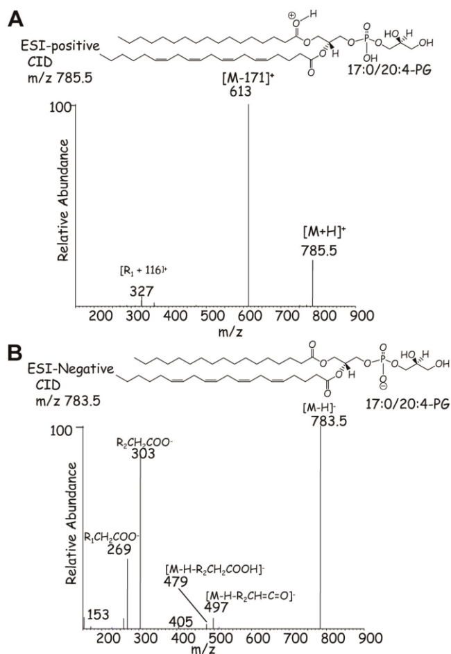
FIGURE 9. Positive and negative ion CID mass spectra from 1-heptadecanoyl-2-arachidonoyl-3-glycerophosphoglycerol (17:0/20:4-PG). Molecular ion species generated by ESI. A: Collisional activation of the [M+H]^+ ion at m/z 785.5; (B) collisional activation of the [M-H]^- ion at m/z 783.5.
